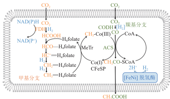
图3 还原性乙酰辅酶A途径示意图 Fig. 3 Schematic diagram of the reductive acetyl-CoA pathway
